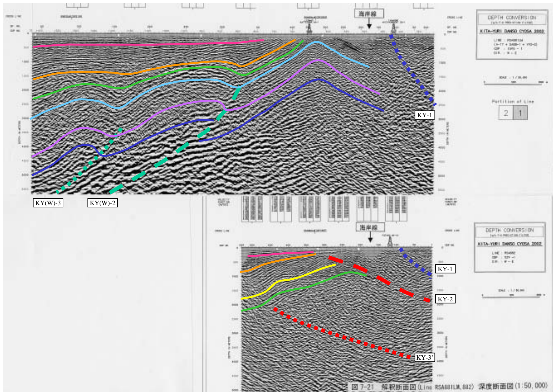
图7-21 解释断面图(RSA881LM-882)
